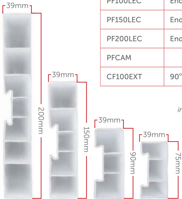
Flexible Boards
