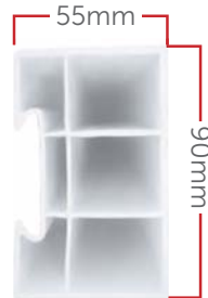
Rigid Board
